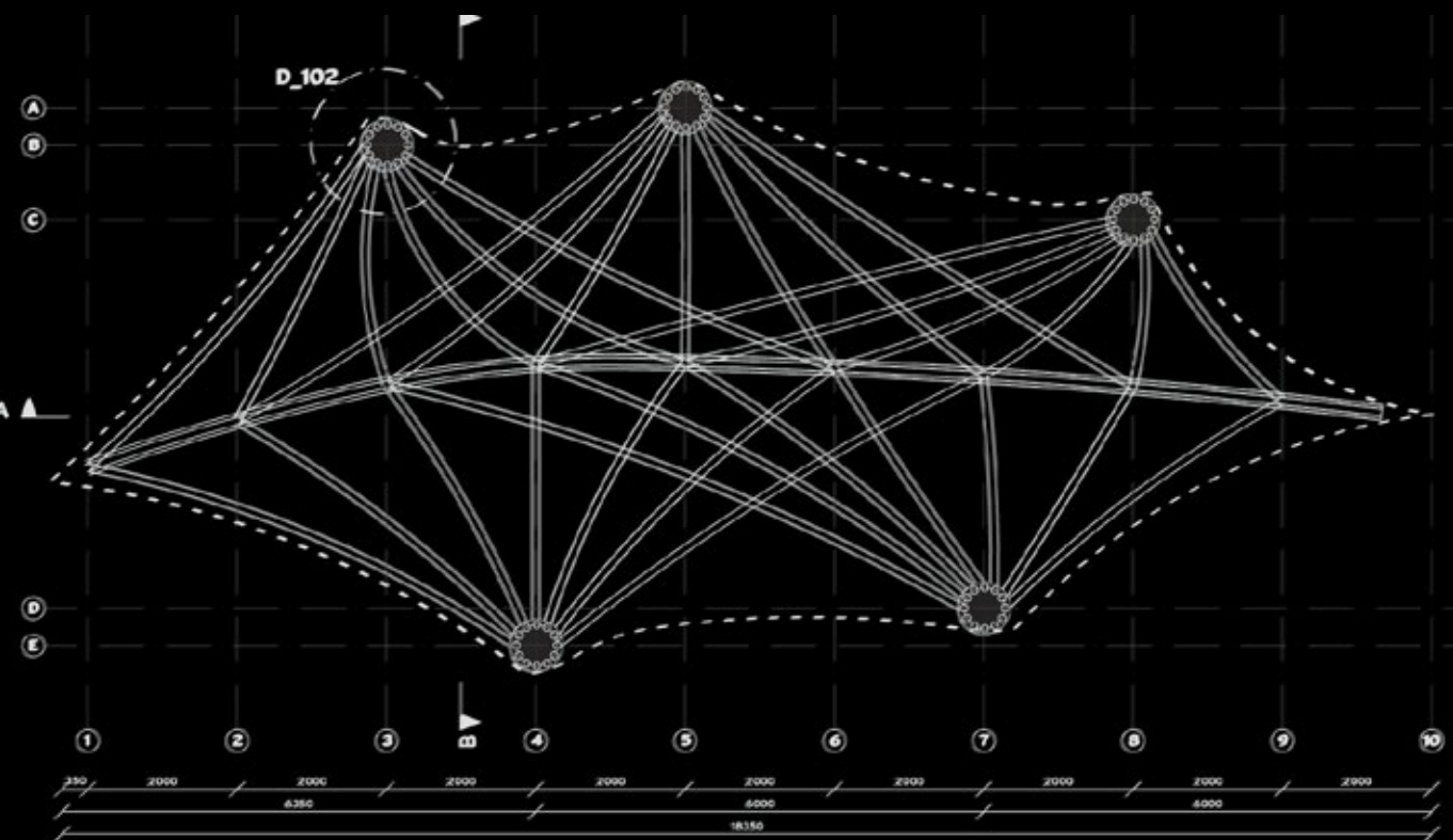
plan main structure
