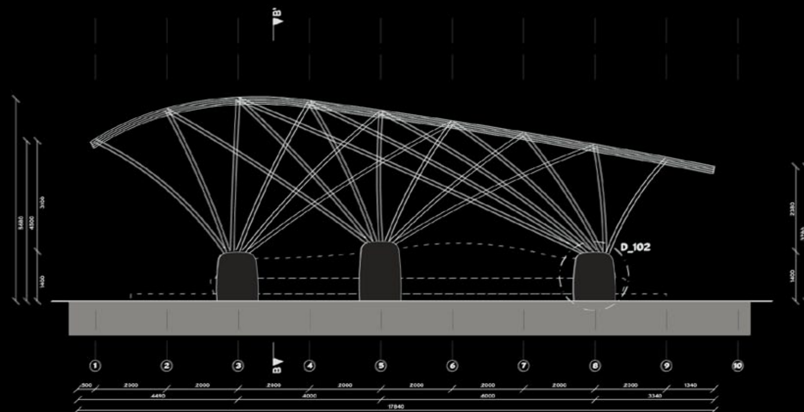
section AA' main structure
