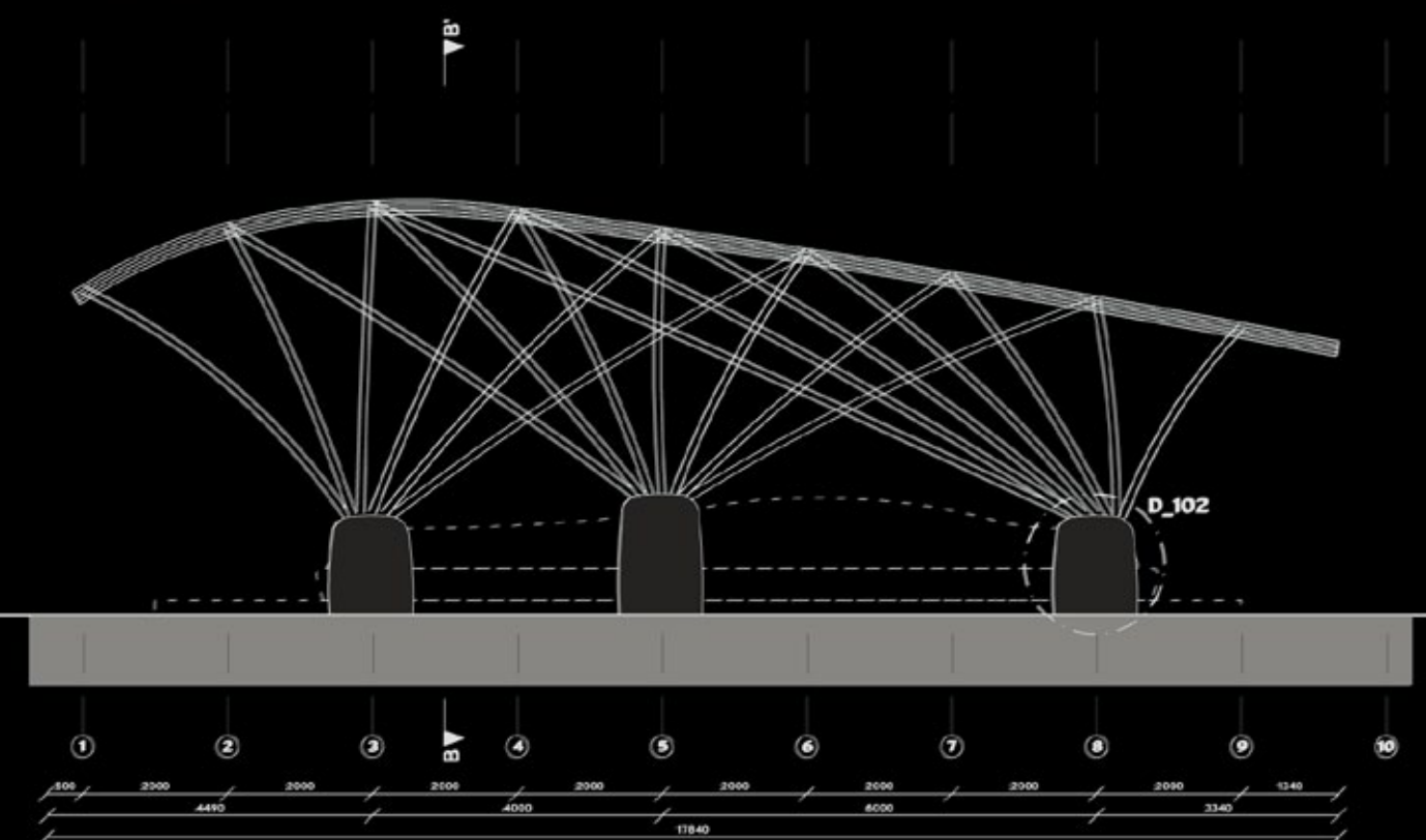
section AA' main structure
